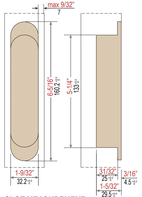
SLOT MEASUREMENT
