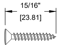
2 - #6 X 15/16" WOOD SCREW
