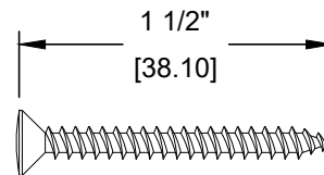
3 - #8 X 1-1/2" WOOD SCREW
