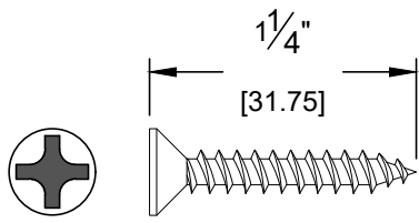
8 - #12 X 1-1/4" WOOD SCREW
