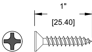
6 - #9 X 1" WOOD SCREW
