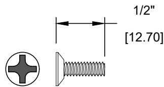
6 - M5 X 1/2" SCREW
