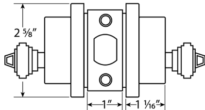
SQ-330 DOUBLE CYLINDER
