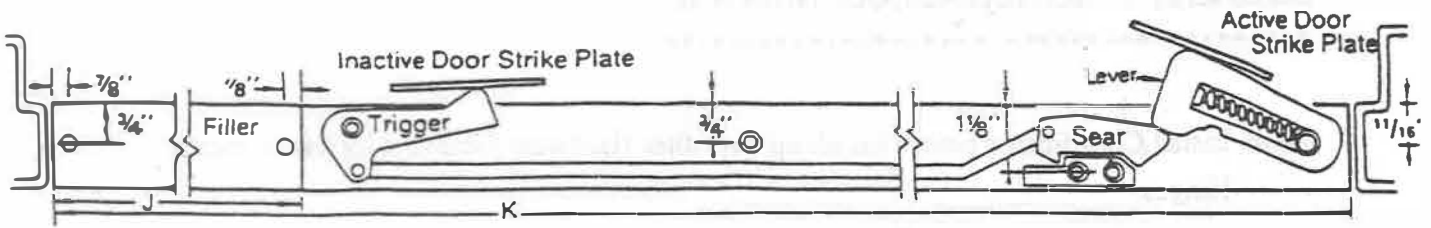
Fig. 3. Coordinator with Filler Bar Doors in open position.
