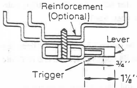
Fig. 5. Doors in open position, Lever and Trigger projection
