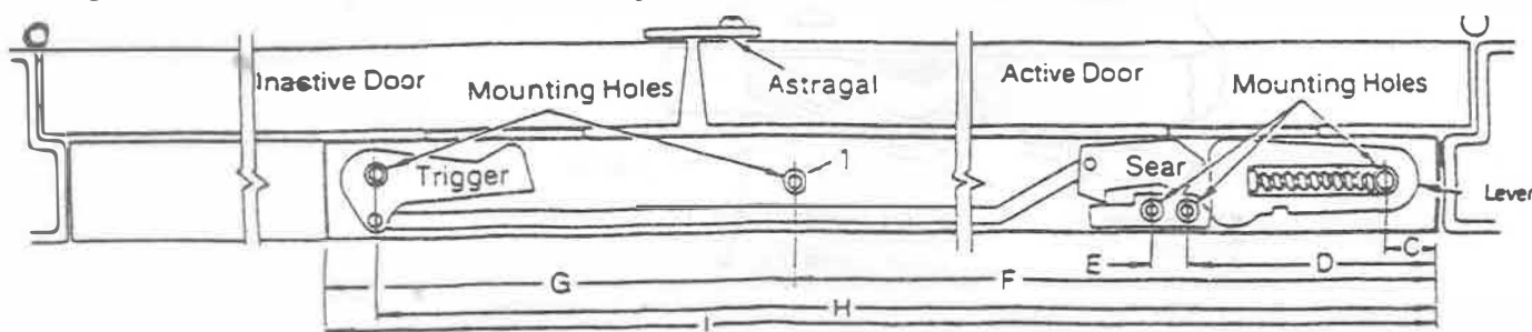
Fig.2. Coordinator with doors in closed position
