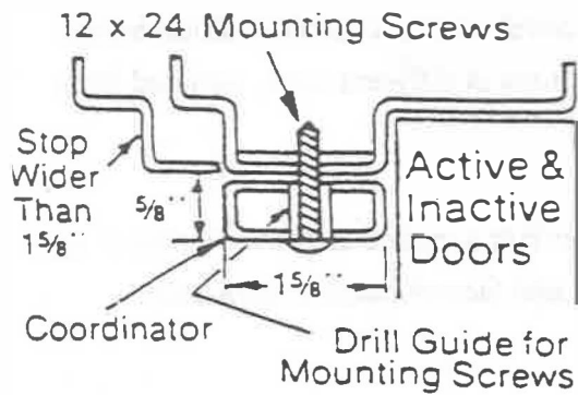
Fig. 4. Doors in closed position
