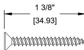
3 - #7 X 1-3/8" WOOD SCREW
