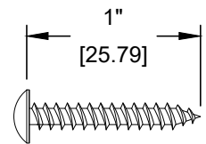
2 - #8 X 1" WOOD SCREW
