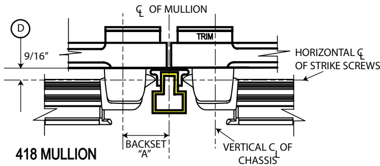
MINIMUM CLEAR STILE REQUIREMENTS TRIM AND MULLION
