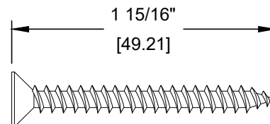
1 - #11 X 1-15/16" WOOD SCREW
