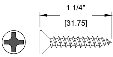
8 - #12 X 1-1/4" WOOD SCREW
